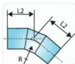
Type 2: Gusseted bend over 31° up to 60°
